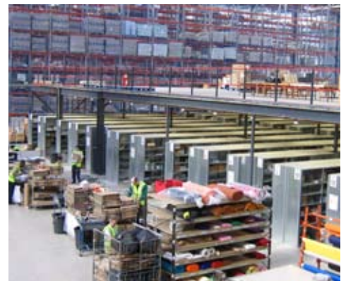
Mezzanine beams, stairways and handrails are designed to conform to the requirements of the latest regulations and make it simple to design and install a first rate storage solution that makes maximum use of the cubic space.
